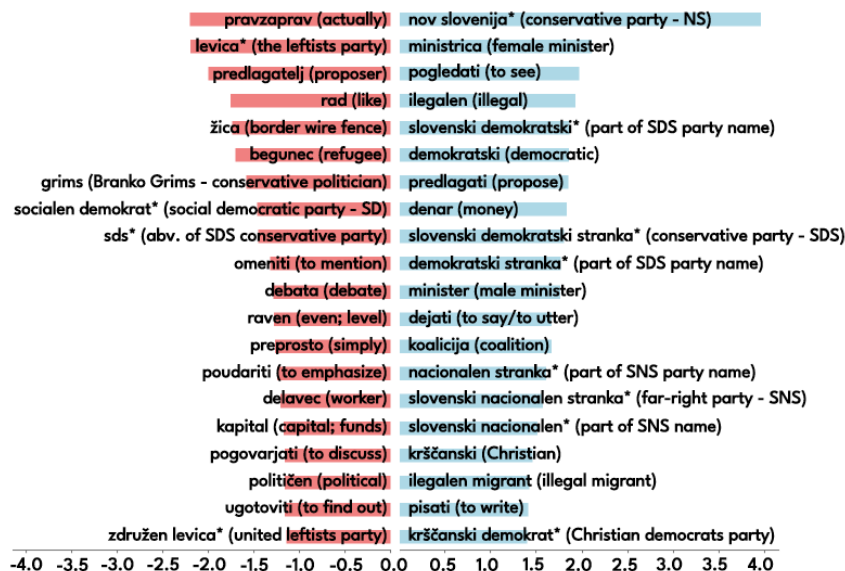
SVM Feature Importance Scale (negative = leftist; positive = rightist)
